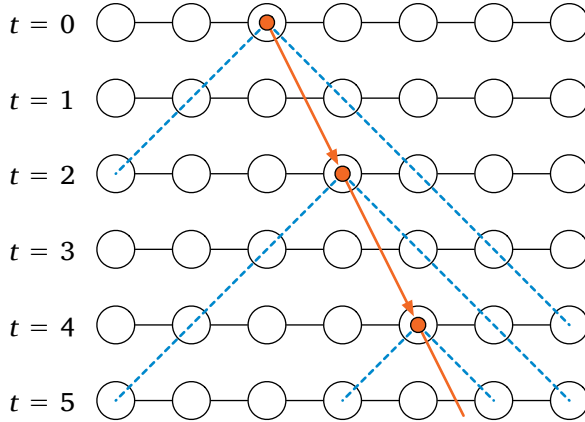
Figure 5.5: Algorithm APSP: the token walks along the BFS tree at speed 0.5 (thick arrows), while each \text{Wave}_v moves along the original graph at speed 1 (dashed lines). The waves are strictly nested: if \text{Wave}_v was triggered after \text{Wave}_u , it will never catch up with \text{Wave}_u .
