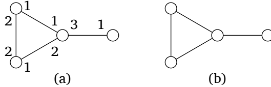
Figure 3.3: (a) An alternative drawing of the simple port-numbered network N from Figure 3.1. (b) The underlying graph G of N .
