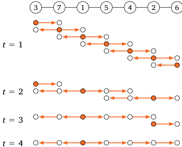
Figure 5.3: Leader election. Each node v will launch a process BFS_v that attempts to construct a BFS tree T_v rooted at v . Other nodes will happily follow BFS_v if v is the smallest leader they have seen so far; otherwise they will start to ignore messages related to BFS_v . Eventually, precisely one of the processes will complete successfully, while all other process will get stuck at some point. In this example, node 1 will be the leader, as it has the smallest identifier. Process BFS_2 will never succeed, as node 1 (as well as all other nodes that are aware of node 1) will ignore all messages related to BFS_2 . Node 1 is the only root that will receive acknowledgments from every child.
